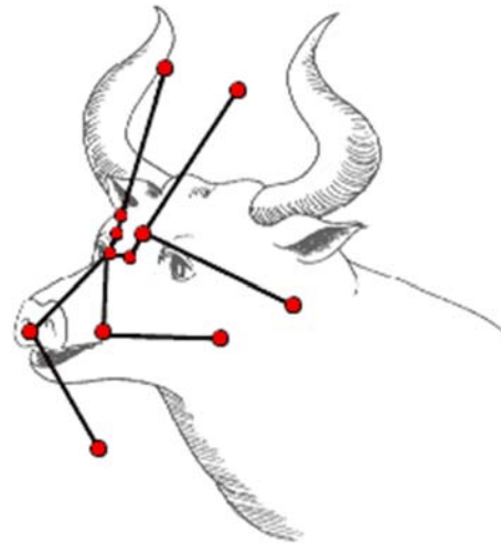
Taurus:
