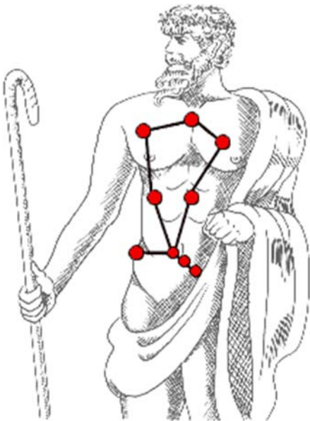
Bootes:
