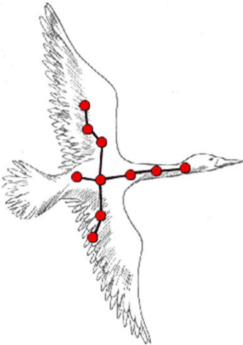
Cygnus:
