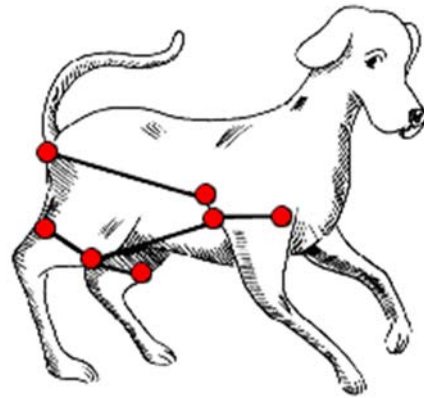
Canis Major:
